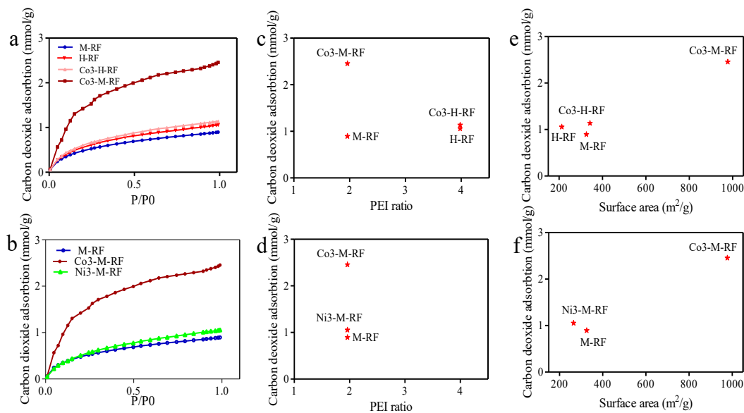
Figure 14. Carbon dioxide absorption of various composition(a-b) at 0 °C (c-d) Carbon absorption at 0 °C and 1 bar verse PEI ratio(e-f) Carbon absorption at 0 °C and 1 bar verse surface area
