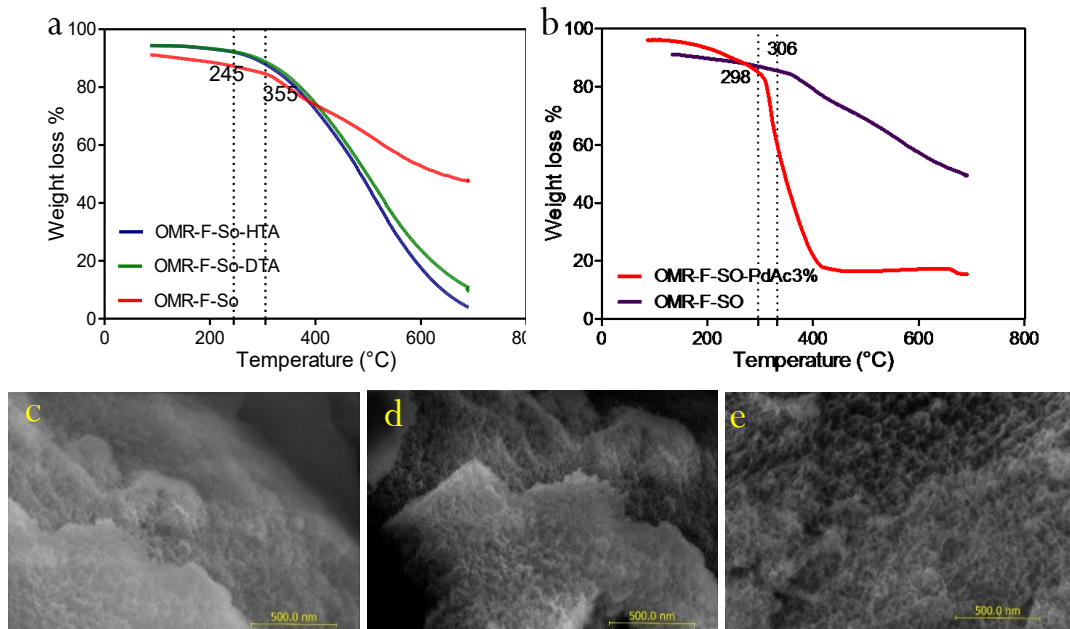
Figure S4 Thermal stability of MR Solvent- template free method with different method and palladium-doped MR solvent-template free method (c-e) SEM images 1. OMR-SO-HTA 2. OMR-SO-DTA 3. OMR-SO
